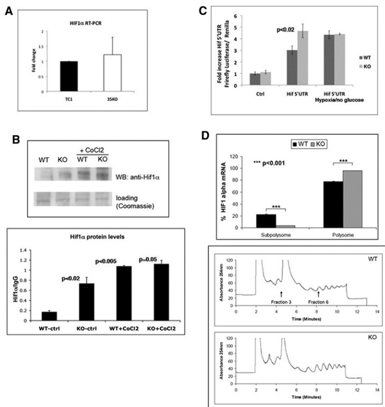
Figure 6. Increased Hif1 \alpha Stability and Protein Synthesis in SIRT6-Deficient Cells
