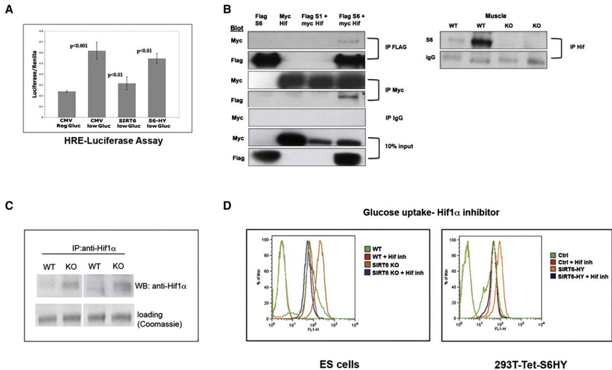
Figure 4. SIRT6 Is a Corepressor of Hif1 \alpha
