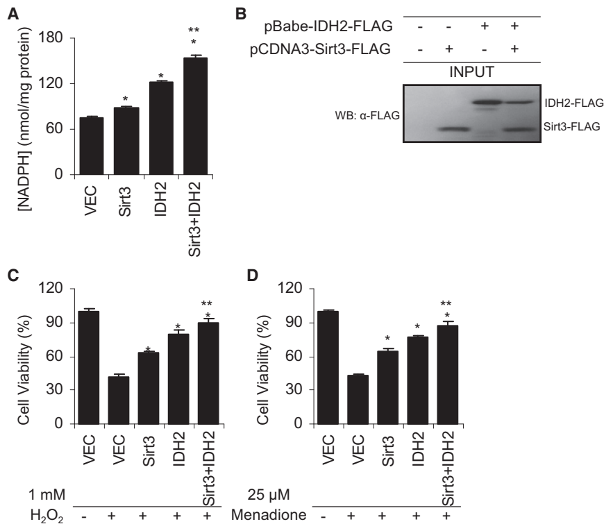
Figure 6. Overexpression of Sirt3 and/or Idh2 Is Sufficient to Increase NADPH Levels and Protects HEK293 Cells from Oxidative Stress
