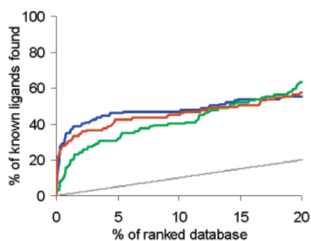
Figure 5. (a) Enrichment plots for PNP obtained from docking (blue line) and rescoring with different charge states assigned to the cofactor phosphate group: \text{H}_2\text{PO}_3^- (orange line), \text{H}_1\text{PO}_3^{2-} (green line), and \text{PO}_3^{3-} (black line). (b) DHFR enrichment results obtained from docking (blue line) and rescoring with incorrectly parametrized ligands (green line) and correctly parametrized ligands (orange line). The incorrectly parametrized ligands have a formal charge of 0 on the pteridine ring.
