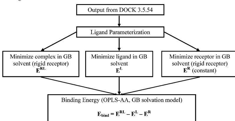
Scheme 1. Refinement and Rescoring Protocol a
