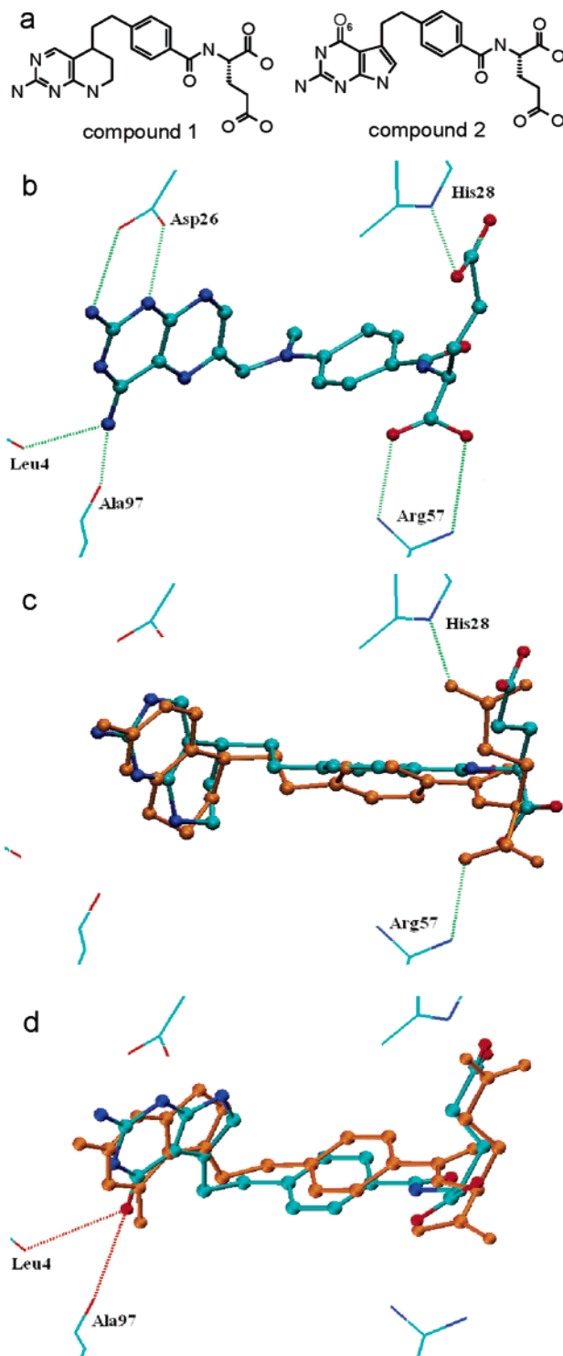
Figure 2. (a) Structures of two DHFR inhibitors, compound 1 and compound 2 , which ranked #1828 and #22 after docking versus #4 and #17 020 after rescoring, respectively. (b) The crystallographic ligand (methotrexate; structure shown in Figure 6a) is represented by a CPK model colored by atom type. The key hydrogen bond interactions between the protein and methotrexate are illustrated with dashed green lines. (c) The docked pose of compound 1 is colored by atom type, while the refined binding pose is in orange. Two hydrogen-bond interactions, identified by dashed green lines, are recovered after minimizing the ligand during the refinement stage. (d) The docked pose of compound 2 is colored by atom type, while the refined binding pose is in orange. The unfavorable interactions between backbone oxygen atoms of protein residue binding site residues and the O6 atom of compound 2 are illustrated with dashed red lines. Molecular images were generated with VMD. 73
