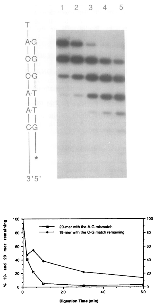
Figure 1. Electrophoretic analysis of terminal mismatch excision by the 3'→5' exonuclease in the Thermococcus litoralis DNA polymerase. The experimental conditions are described under 'methods'. Lanes 1–5 in the autoradiogram represent the Vent TM N DNA polymerase reactions in which the oligonucleotide with the A·G mismatch in the 3'-prime end of the primer terminus was used as substrate for the exonuclease. Incubation was for 2, 5, 10, 30 and 60 min, respectively. The lower part of the picture is a plot of the data obtained by excising each fragment from the gel and counting the radioactivity with a scintillation counter.
